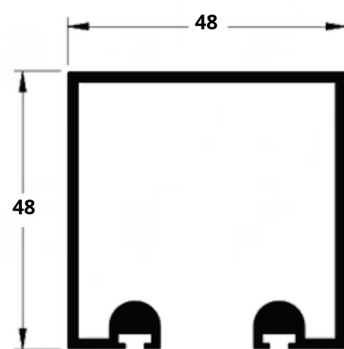
CR-270 1,151 Kg/m
