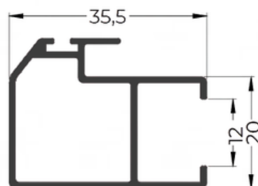
PRM20-F03 0,399 Kg/m
