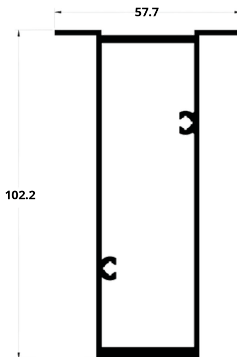
A6 LG-176 1,424 kg/m
